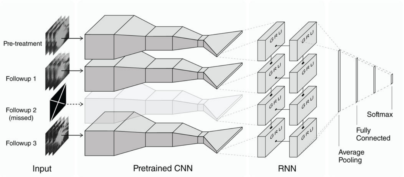
Figure 3: Deep Learning Architectures.
